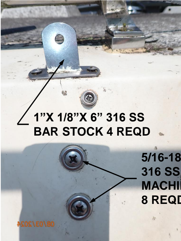
EXTERIOR VIEW PORT SIDE, FRONT LOWER CHAINPLATE & BOLTS
